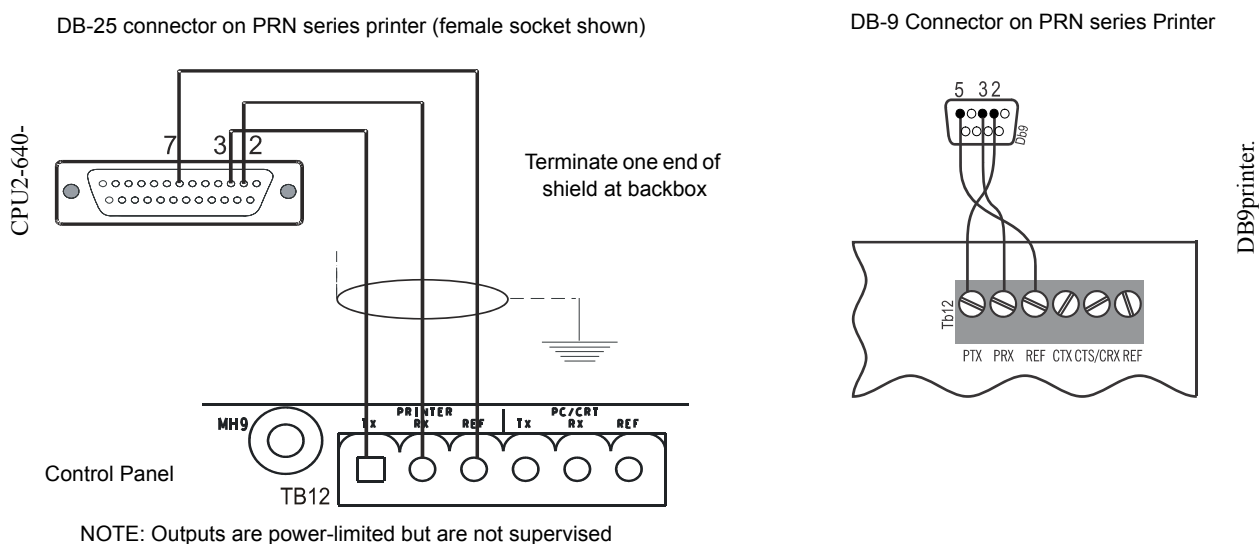
Figure 3.5 Remote Printer Connections
