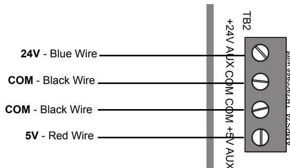
Figure 3.7 Connecting to the Accessories Output TB2 on CPS-24/E
