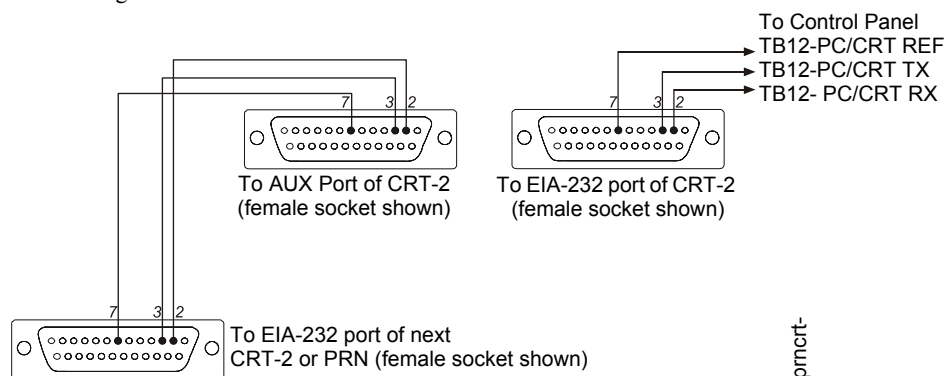
Figure 3.7 Connecting Multiple Devices on the EIA-232 Circuit
