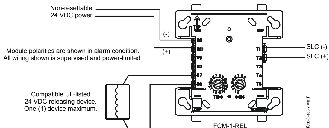
Figure 4.13 NPFA Class B Wiring of the FCM-1-REL
