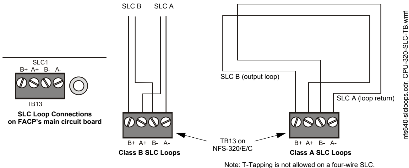
Figure 3.8 SLC Loop Connections and Wiring
