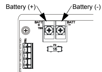
Figure 3.5 CPS-24/E: DC Power Connections
