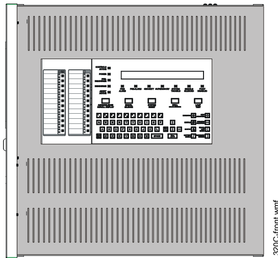
Figure C.1 NFS-320C, Shown in its Dress Panel with Door Open
