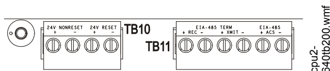
Figure 3.4 EIA-485 Connections
