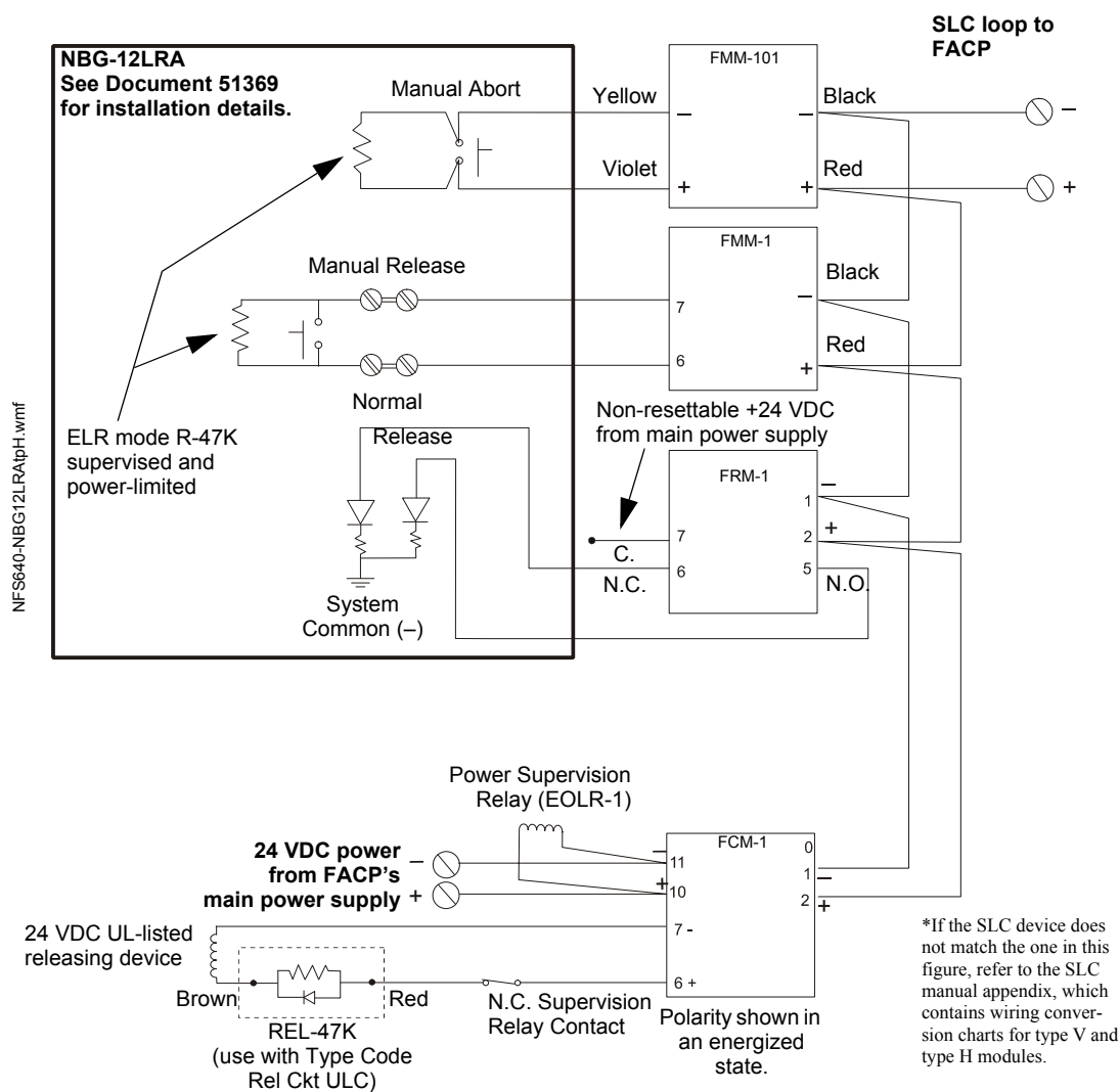
Figure 4.14 Typical Connections for an NBG-12LRA Agent Release-Abort Station
