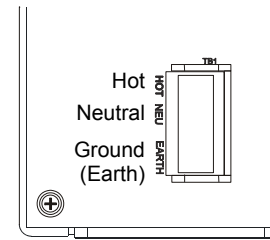
Figure 3.4 CPS-24/E: AC Power Connections
