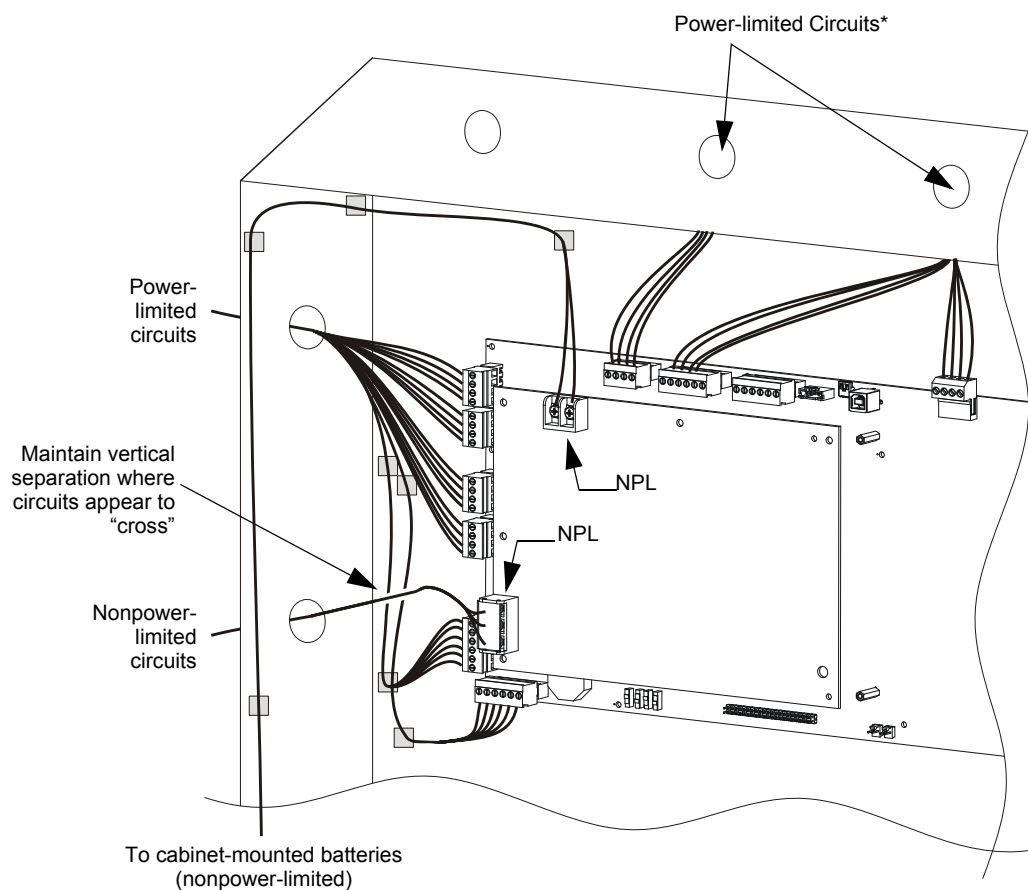
Figure 3.3 Typical Wiring for UL Power-limited Wiring Requirements (Shown with relays as connected to power-limited modules)
