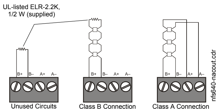
Figure 3.8 Notification Appliance Circuit (NAC) Connections
