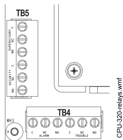
Figure 3.1 Form-C Relay Connections
