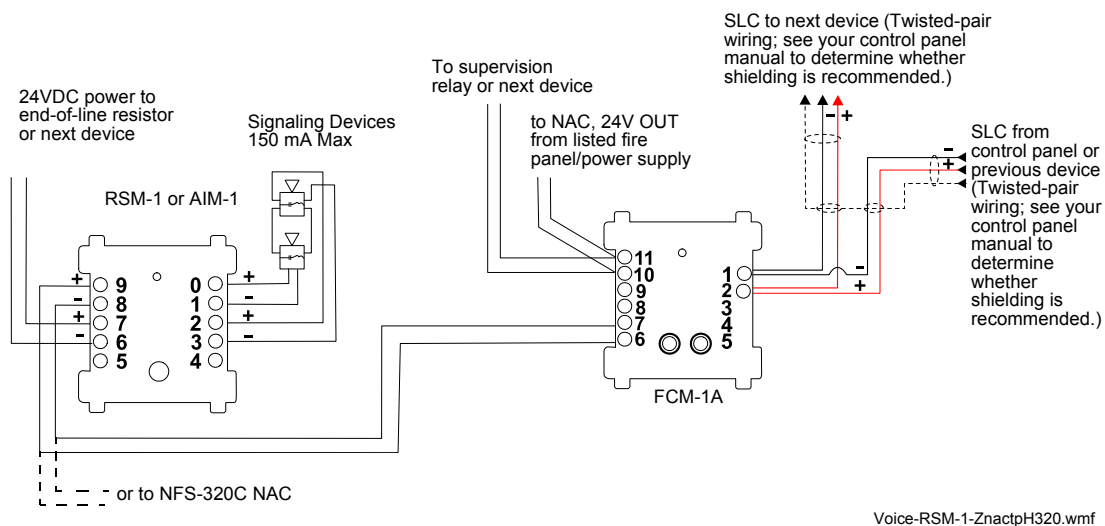
Figure 4 RSM-1/AIM-1 NAC Connections, Supervised, Class A
