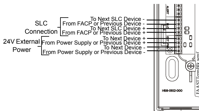
Figure 4 FSA-8000 Connection to the FACP
