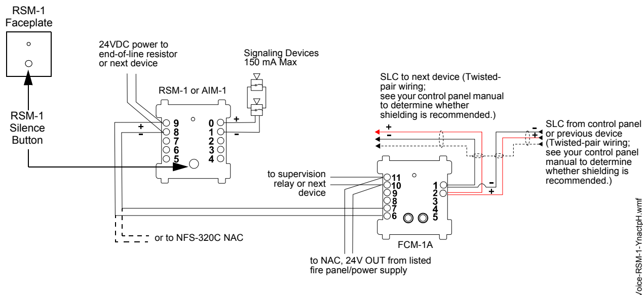
Figure C.1 RSM-1/AIM-1 NAC Connections, Unsupervised, Class B
